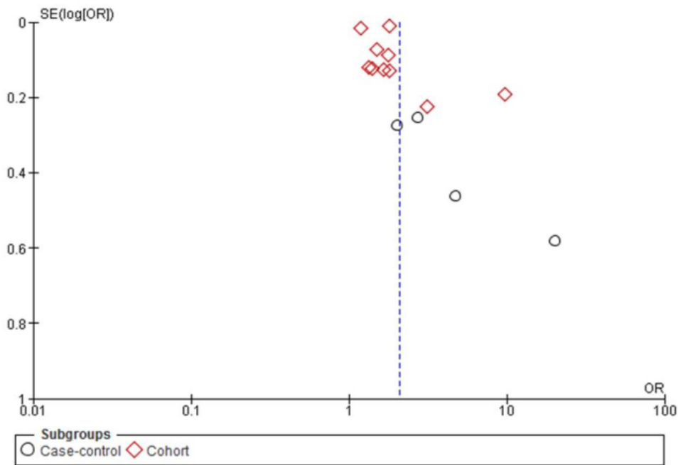
Fig. 2 Funnel Plot
