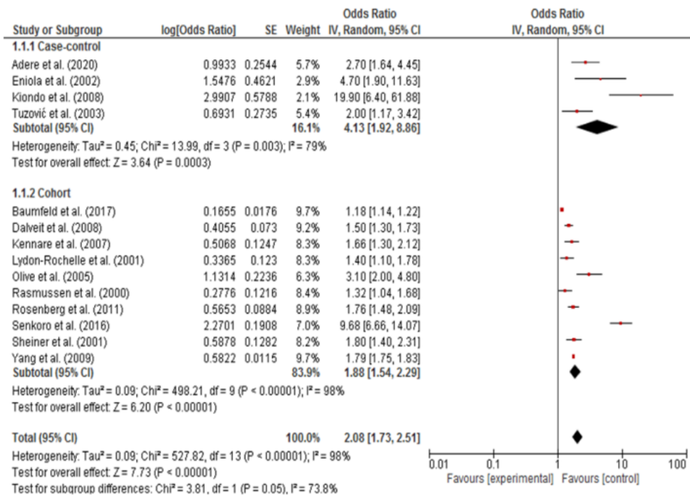
Fig. 1 Forest Plot
