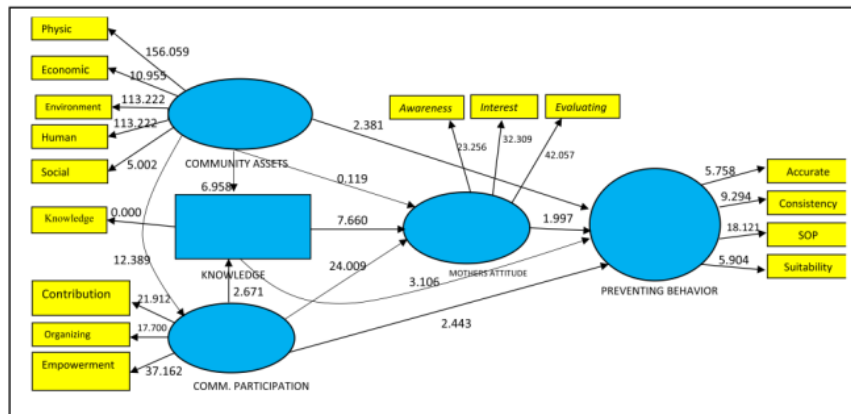
Figure 7. T Statistik of YUDHIA Model
