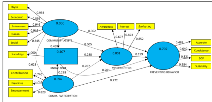
Figure 6. Factor Loading of YUDHIA Model
