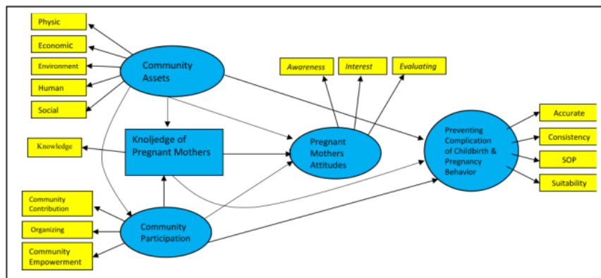
Figure 5. YUDHIA Model Structural with SEM PLS
