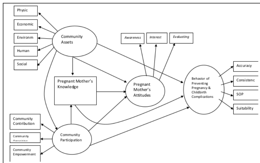
Figure 2. Conceptual Framework for Equation Model
