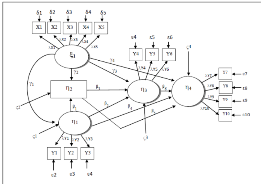
Figure 3. Analysis Framework with Structural Equation Model
