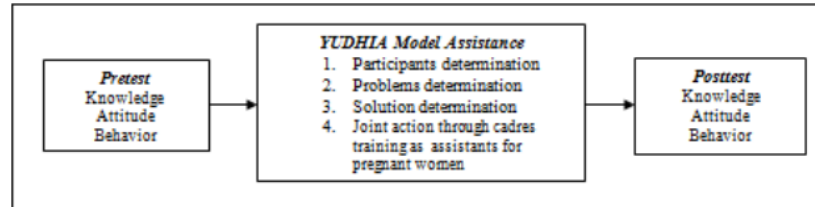
Figure 4 YUDHIA Model evaluation concept framework
